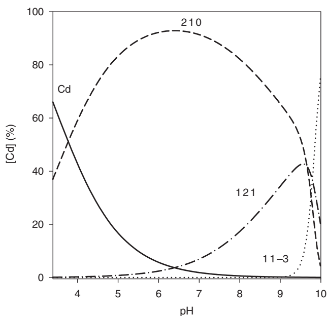
Figure 3. Species distribution for the \text{Cd}^{2+}/\text{cnge (L)}/\text{H}^+ system. Total concentrations: \text{Cd}^{2+} , 0.1 \text{ mmol L}^{-1} and \text{cnge} , 0.2 \text{ mmol L}^{-1} as a function of pH, 25^\circ\text{C} , I=0.150 \text{ mol L}^{-1} NaCl.
