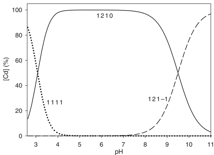
Figure 4. Species distribution for the \text{Cd}^{2+}/\text{o-phen (A)}/\text{cnge (L)}/\text{H}^+ system. Total concentrations: \text{Cd}^{2+} , 0.5 \text{ mmol L}^{-1} , \text{phen} , 1.5 \text{ mmol L}^{-1} and \text{cnge} , 1 \text{ mmol L}^{-1} as a function of pH, 25^\circ\text{C} , I=0.150 \text{ mol L}^{-1} NaCl.
